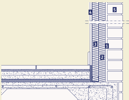
1. Mortero 2. URSA TERRA Plus 32 T003 3. URSA TERRA Mur P1281 4. PYL 5. Pared de ladrillo
